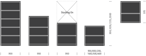
CK2 Open Shelf Cabinet
