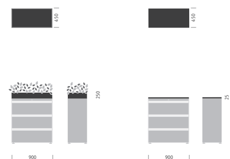
Planter For CK2 & CK8 Cabinet
