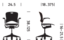
Multipurpose Chair with Molded Back and Seat
