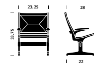
Single Seat Dimensions
