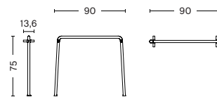
PALISSADE MIDDLE LEG LENGTH 90 CM | 35.43" DEPTH 13,5 CM | 5.31" HEIGHT | 75 CM | 29.53"
