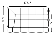
QLT2L | WIDE MODULE | LEFT WIDTH 176,5 CM | 69.88" DEPTH 109 CM | 43.5" HEIGHT 72 CM | 28.5" SEAT HEIGHT 41 CM | 16.25" SEAT DEPTH 77 CM | 30.25"
