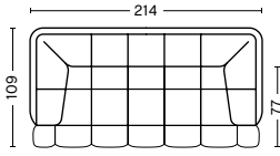
QLT1A | 2 SEATER WIDTH 214 CM | 84.25" DEPTH 109 CM | 43.5" HEIGHT 72 CM | 28.5" SEAT HEIGHT 41 CM | 16.25" SEAT DEPTH 77 CM | 30.25"
