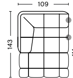
QLT5L | CHAISE LONGUE MODULE | LEFT WIDTH 109 CM | 43" DEPTH 143 CM | 56.25" HEIGHT 72 CM | 28.5" SEAT HEIGHT 41 CM | 16.25" SEAT DEPTH 111 CM | 43.75"
