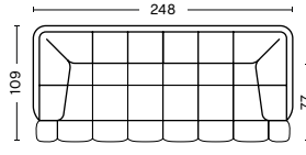
QLT2A | 2.5 SEATER WIDTH 248 CM | 97.5" DEPTH 109 CM | 43.5" HEIGHT 72 CM | 28.5" SEAT HEIGHT 41 CM | 16.25" SEAT DEPTH 77 CM | 30.25"
