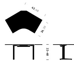
120° Corner Table with C-Foot
