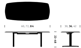
Oval Table with T-Foot
